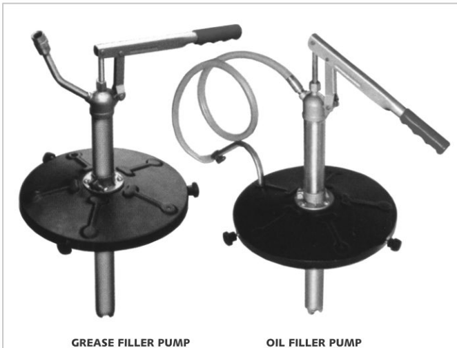
GREASE FILLER PUMP
